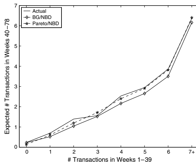
Figure 3 Conditional Expectations
